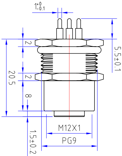
LATERAL VIEW
