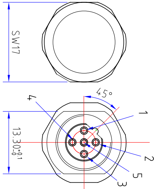
FRONTAL VIEW
