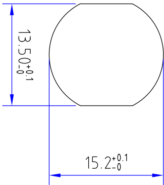
PANEL CUT
