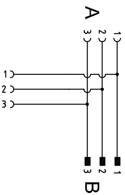
ELECTRICAL SCHEME
